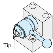
Sideways Clamping
